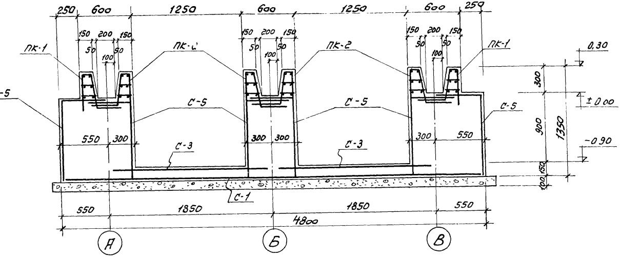
III - III
