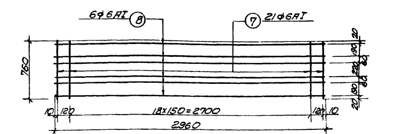
C-8
