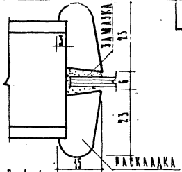
No 4-4
