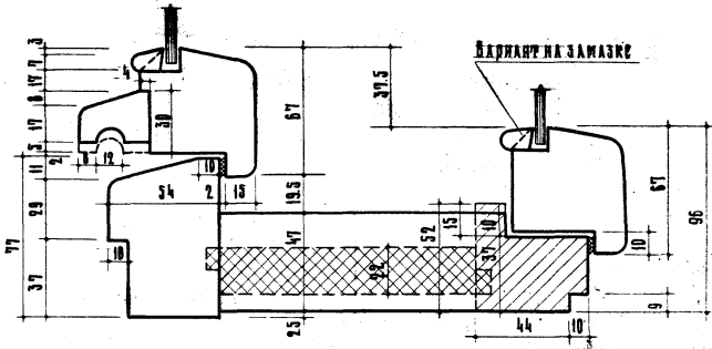
По 3-3
