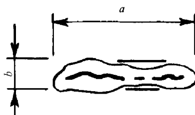
2: a/b \geq 3
