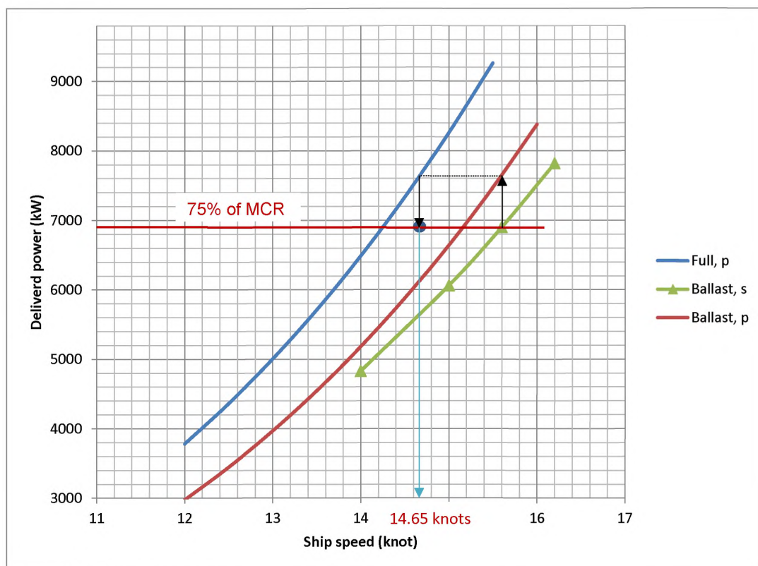
Figure 3.1: Power curves
