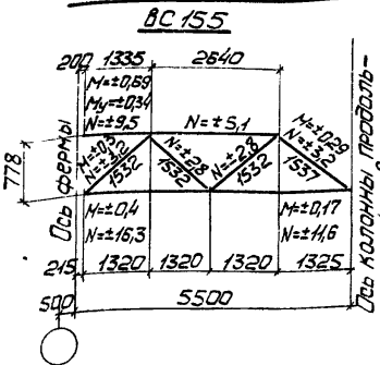
BC 155, BC 156
