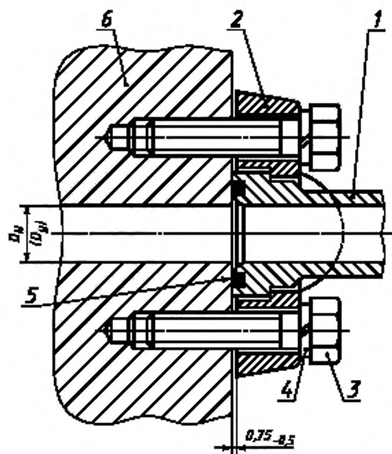
1 — nipple; 2 — two detachable semi-flanges; 3 — bolt; 4 — spring washer; 5 — rubber ring; 6 — housing (nest)
